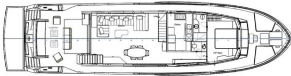
Main Deck
