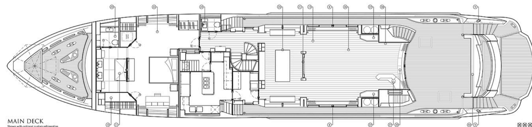
MAIN DECK
