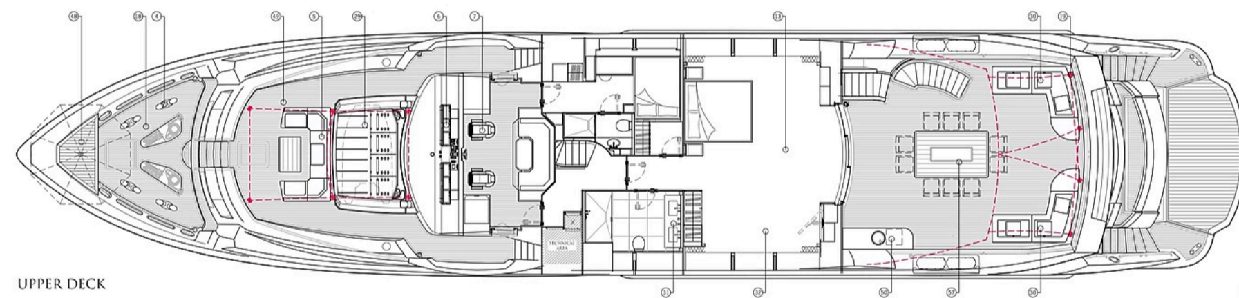
SKYDECK
