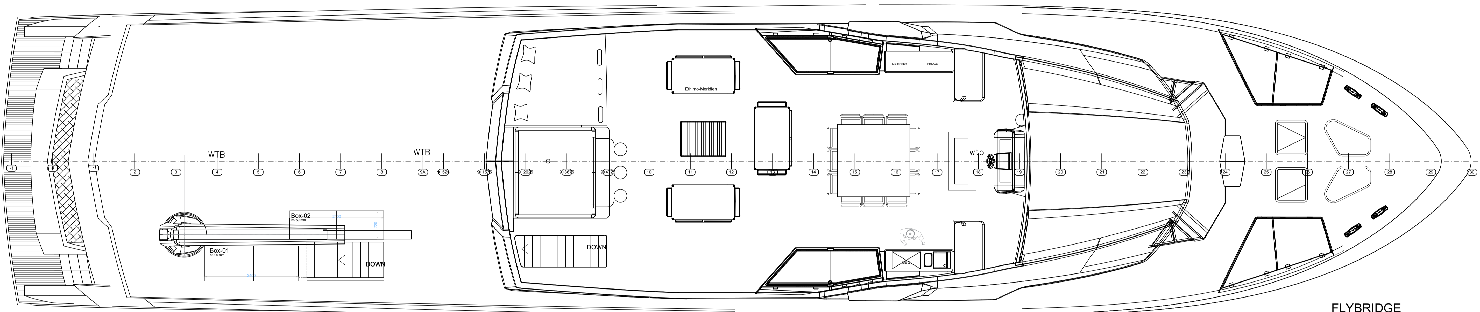
FLYBRIDGE DECK
